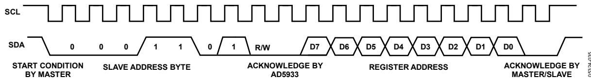
Figure 35. Timing Diagram
