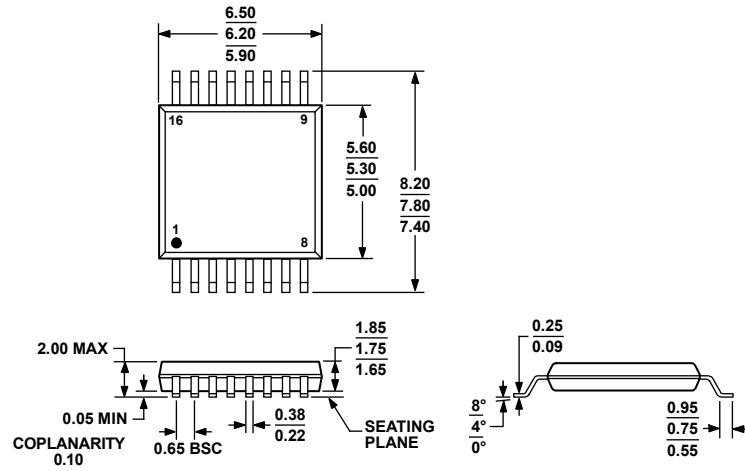
Figure 49. 16-Lead Shrink Small Outline Package [SSOP] (RS-16)
